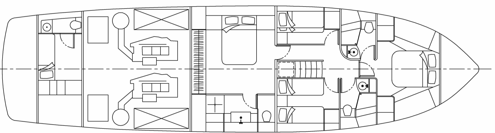
LOWER DECK PLAN
