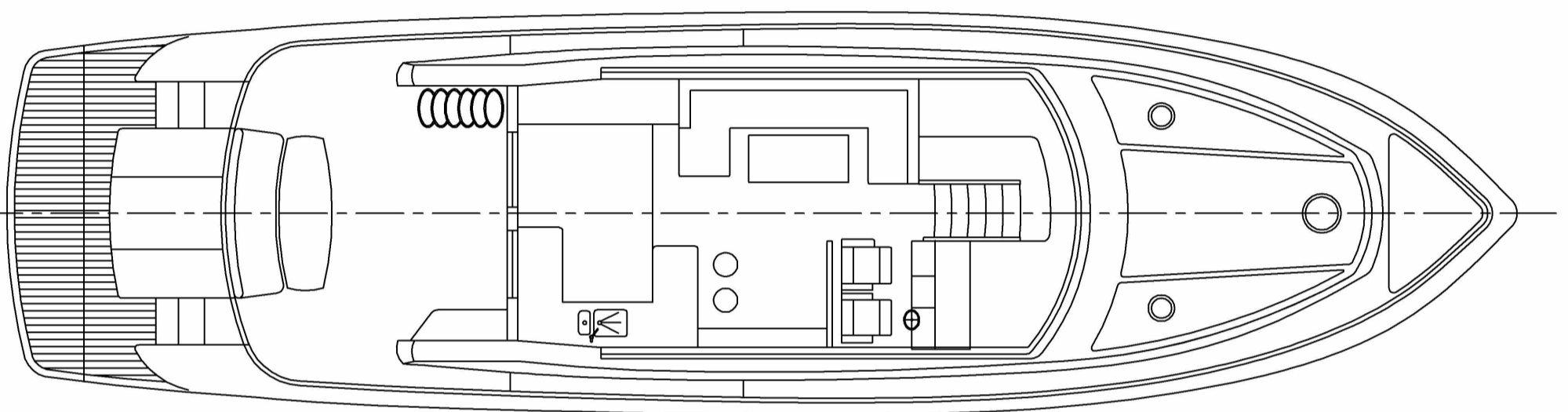
MAIN DECK PLAN
